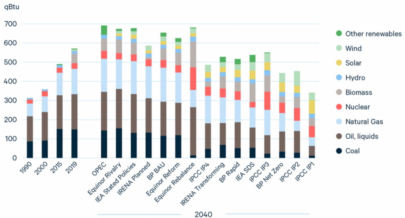
Global primary energy fuel shares in 2040
